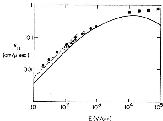
FIG. 1. Field dependence of the drift velocity of electrons in liquid argon. Squares—data of D. W. Swan [Proc. Phys. Soc. (London) 83 , 659 (1964)]; triangles—data from Ref. 1, taken at 85°K; circles—present work, obtained at 85°K with two cells. The line is the single-scatterer theory taken from Ref. 5, and the dashed line is the same corrected for multiple scattering in the Ohmic region.
