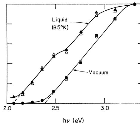
FIG. 2. Photoemission yields in vacuum and in liquid, per unit light intensity. The extrapolated curves meet the energy axis at 2.39 and 2.06 eV. Each set of points is the average of three runs. The origin of the kink in the liquid curve between 2.5 and 2.6 eV is not known; it is reproducible and persists when a tungsten-filament lamp is used as light source.
